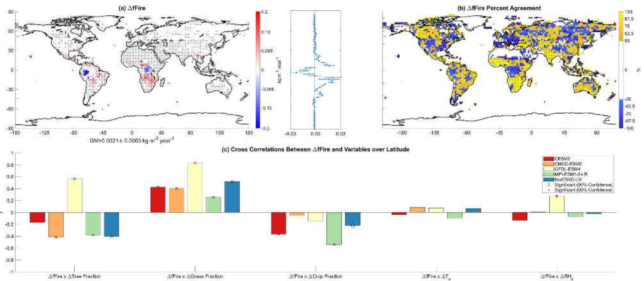
Fig. 7 | Change in fire carbon emissions under net forestation (ssp370-ssp126Lu – ssp370) over years 2070–2099. Multi-model annual mean response of (a) fire carbon emissions ( fFire ; kg\ m^{-2}\ year^{-1} ). The global mean change and uncertainty are indicated underneath panel (a). Black dots in (a) symbolize statistically significant differences at the 95% confidence interval using a two-tailed test. Depicted to the right of (a) is a zonal mean of fFire , with the uncertainty based on the 95% confidence interval of the model spread. b Model percent agreement on the sign of the fFire
